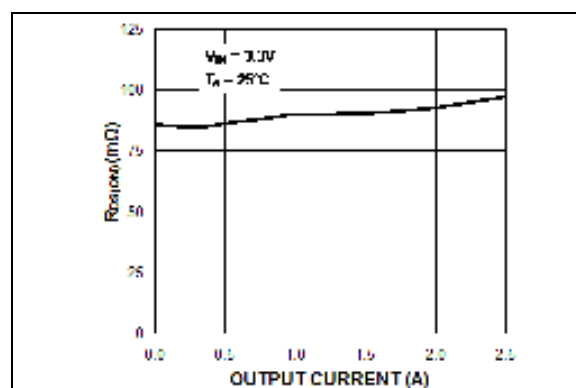
FIGURE 2-6: R_{DS(ON)} vs. Output Current.
