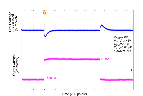
FIGURE 2-30: LDO Load Transient LowQ Mode.
