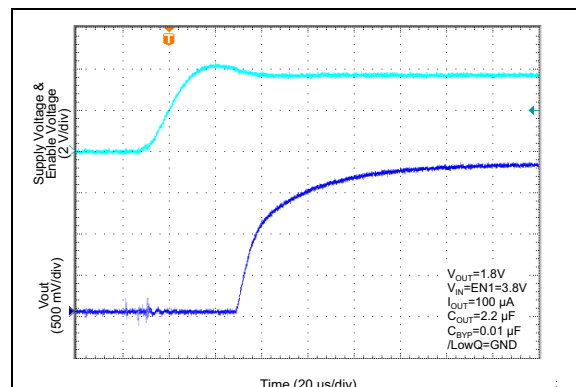
FIGURE 2-28: Enable Transient LowQ Mode.
