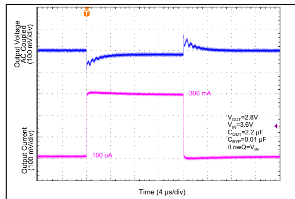
FIGURE 2-29: LDO2 Load Transient Normal Mode.
