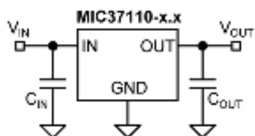
Figure 1. Capacitor Requirements
