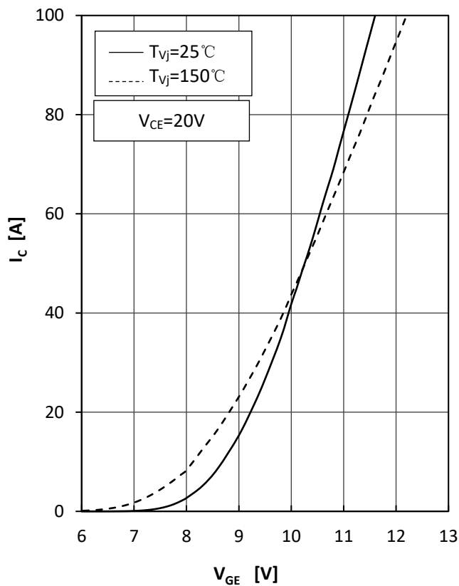
Fig2.IGBT Transfer Characteristics
