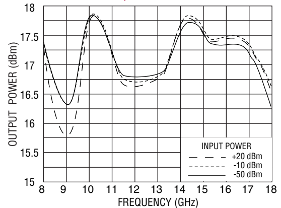
TYPICAL PERFORMANCE OF MITEQ LIMITING AMPLIFIER (OUTPUT POWER VS. INPUT POWER)
