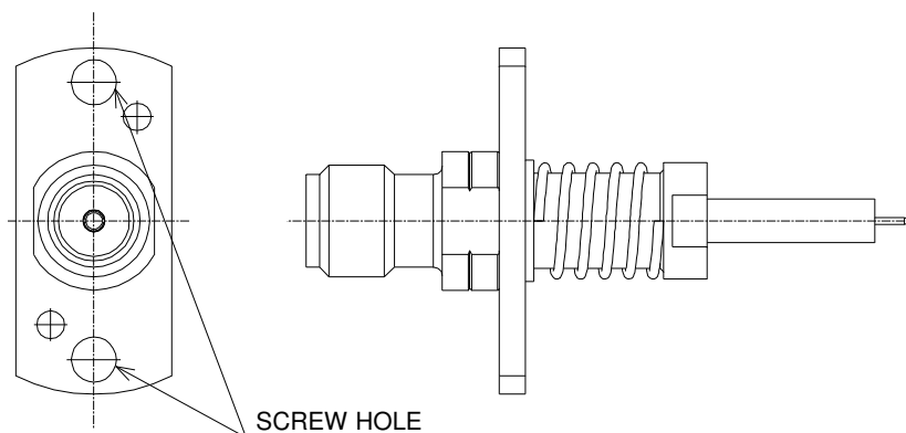
Figure.2 Screw hole position
