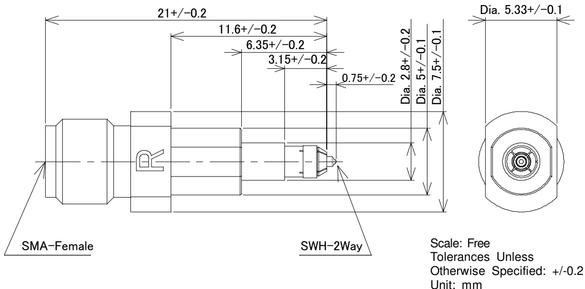
Figure.1 Construction
