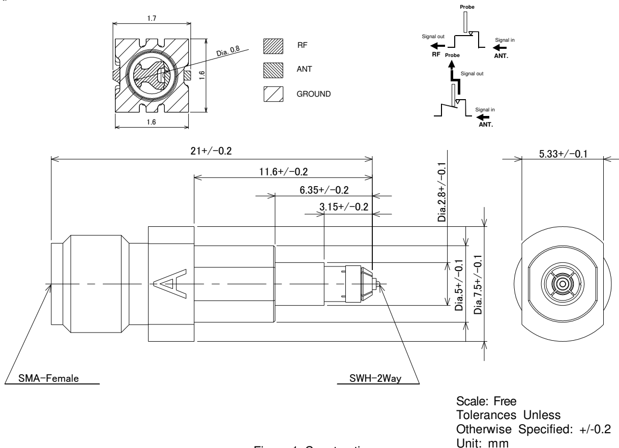
Figure.1 Construction
