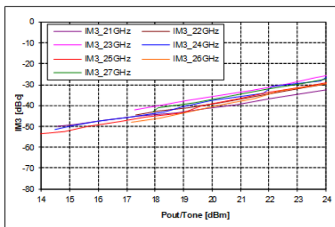
IM3 Level vs. single tone output power [dBm/ton]
