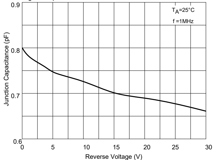
Fig. 3 - Capacitance Characteristics
