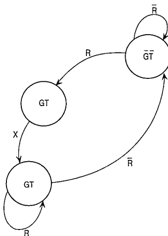
(b) 2-Wire Bus Arbitration Figure 5-18. Bus Arbitration Unit State Diagrams
