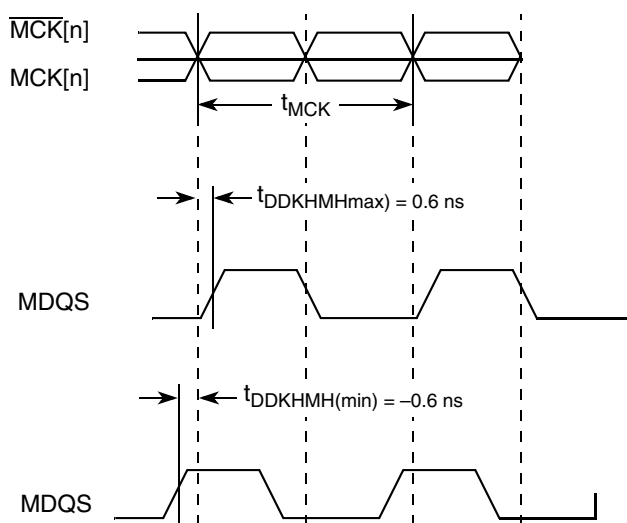
Figure 6. Timing Diagram for t_{DDKMH}
