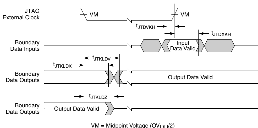
Figure 47. Boundary-Scan Timing Diagram
