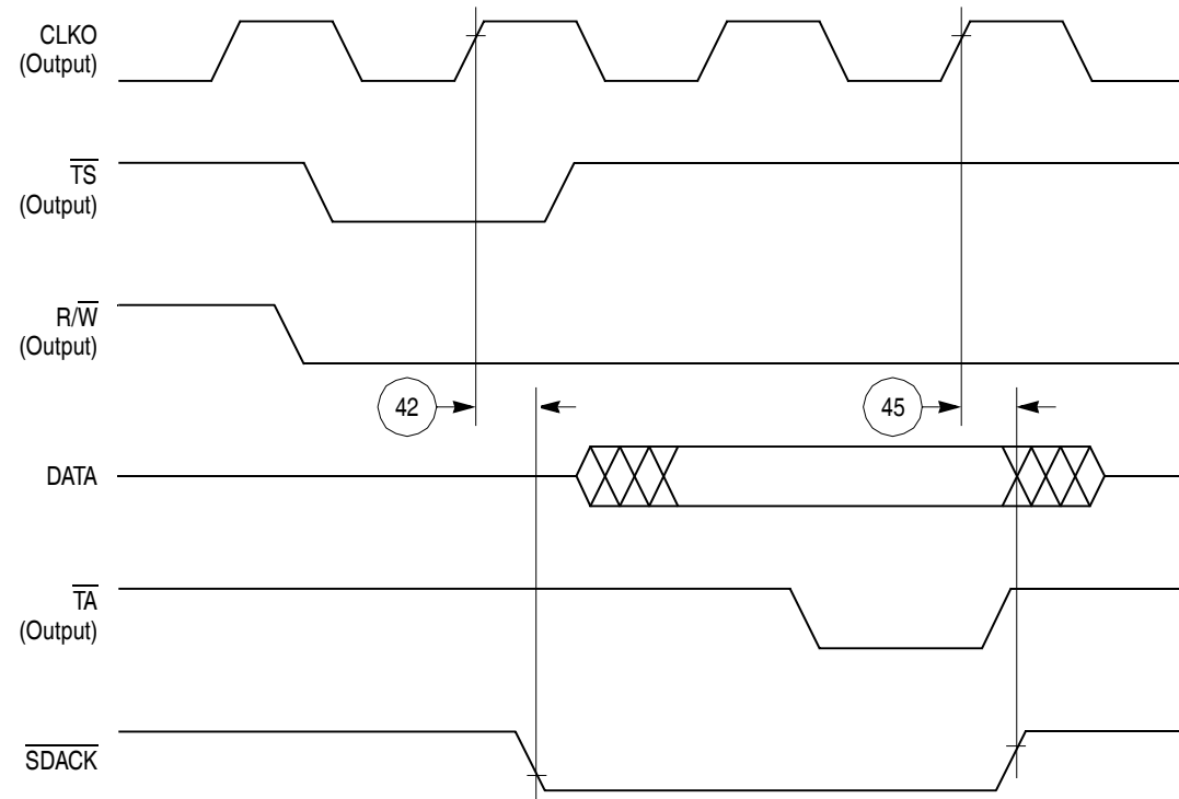
Figure 49. \overline{SDACK} Timing Diagram—Peripheral Read, Internally-Generated \overline{TA}
