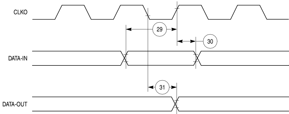
Figure 44. Parallel I/O Data-In/Data-Out Timing Diagram
