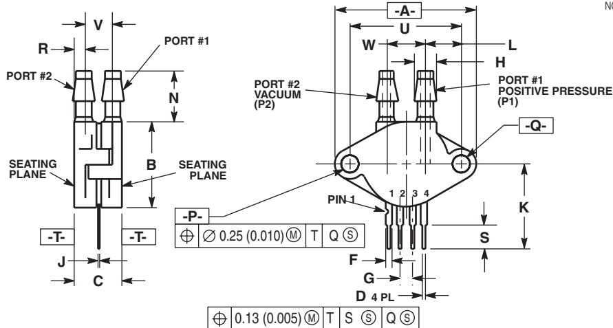
CASE 344C-01 ISSUE B UNIBODY PACKAGE
