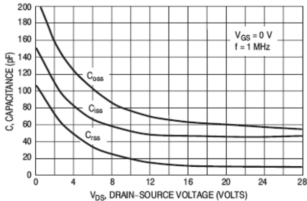
Figure 12. Capacitance versus Drain-Source Voltage
