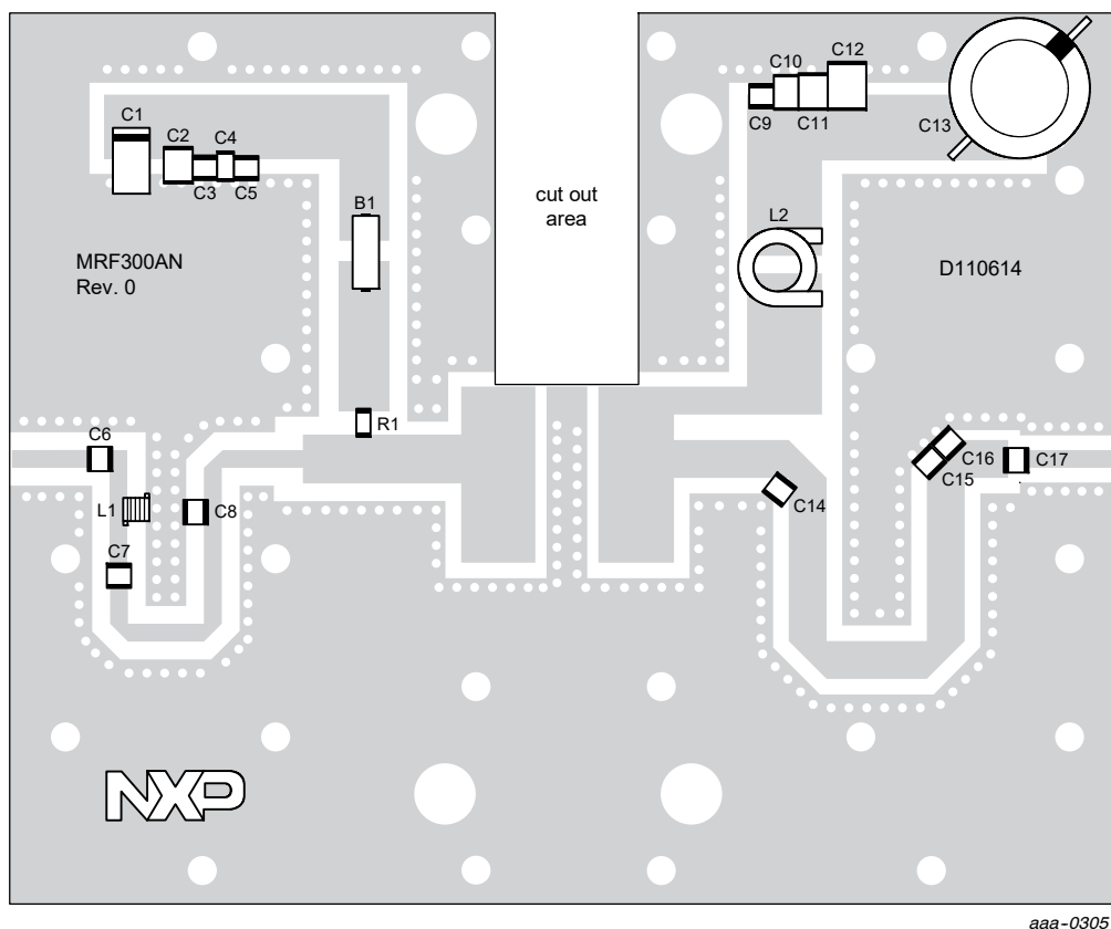
Figure 8. MRF300AN Fixture Component Layout — 230 MHz
