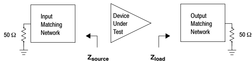
Figure 14. Series Equivalent Source and Load Impedance — 230 MHz
