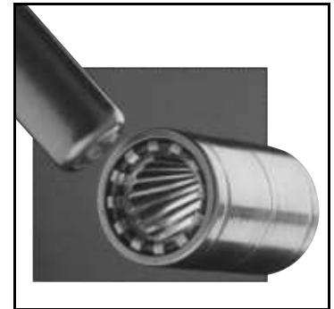
The RADSOK design - socket cylinder within female contact has twisted hyperbolic grid. Provides higher amperage capabilities with low insertion force and low temperature rise.
