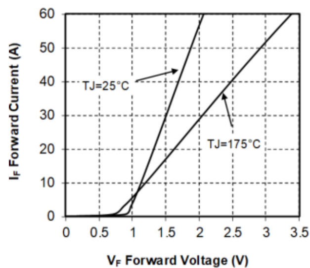
Figure 1-16. Forward Characteristics
