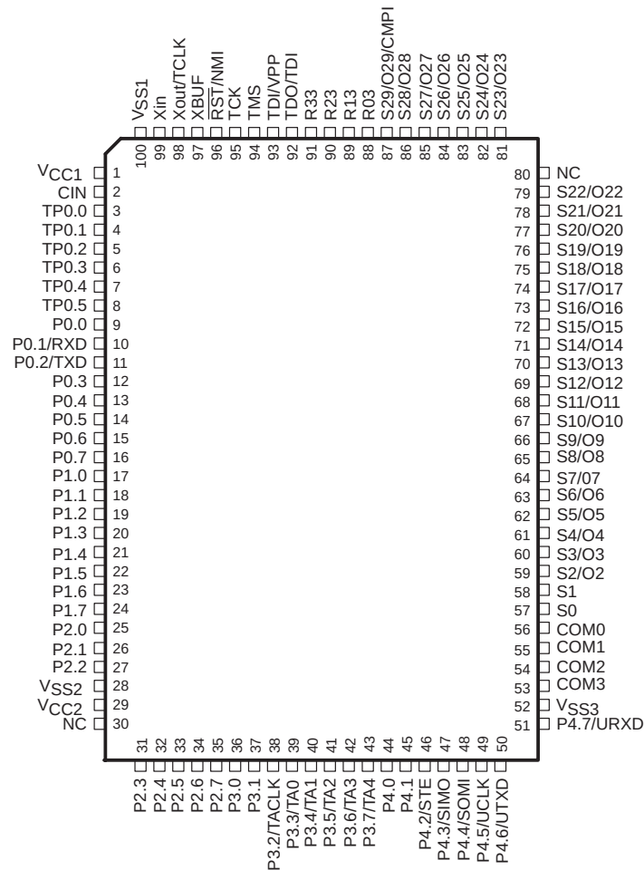
PJM or HFD PACKAGE (TOP VIEW)
