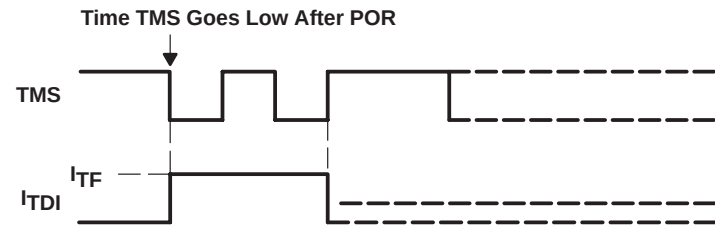
Figure 21. Fuse Check Mode Current, MSP430P337A
