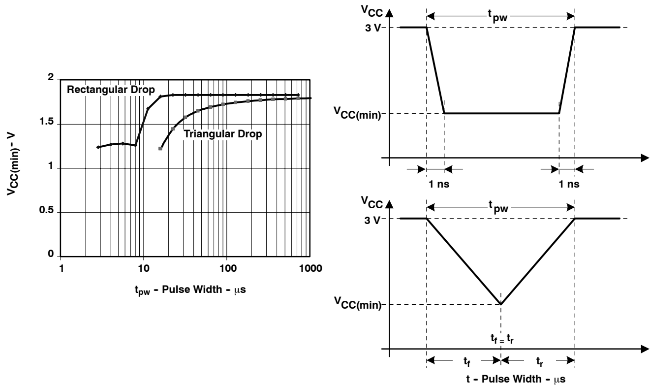
Figure 11. V_{CC(min)} : Square Voltage Drop and Triangle Voltage Drop to Generate an SVD Signal ( VLD = 1 )
