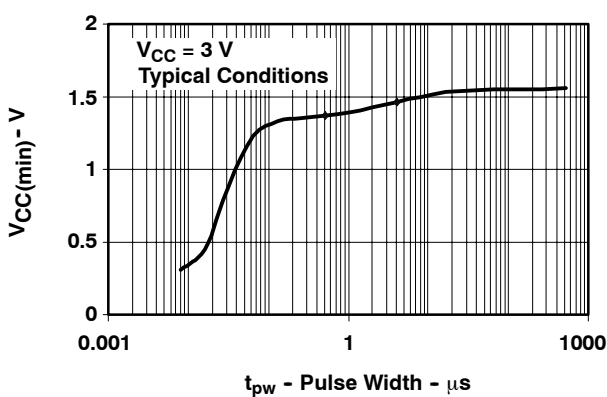
Figure 8. V_{CC(min)} Level With a Square Voltage Drop to Generate a POR/Brownout Signal
