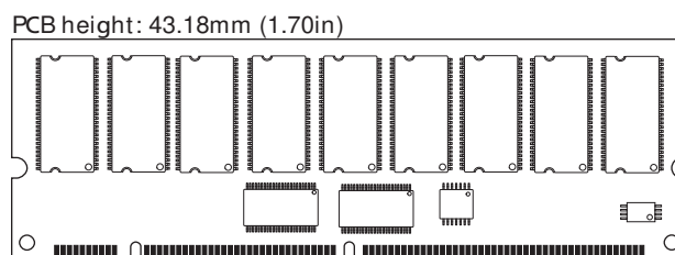
Figure 2: Low Profile Layout (R/C G)
