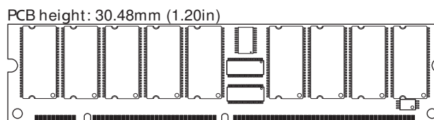
Figure 2: Low Profile Layout (R/C G)
