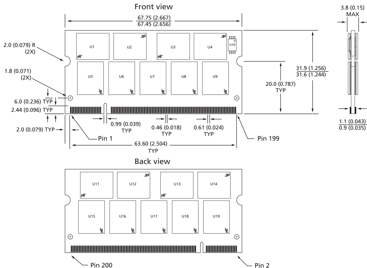
Figure 3: 200-Pin SODIMM
