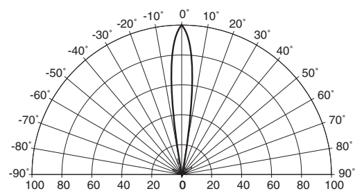
Fig. 4 Radiation Diagram
