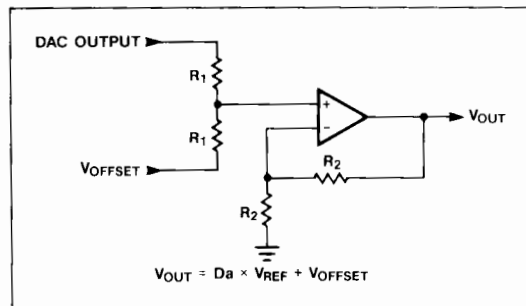
Figure 9. Offset Circuit
