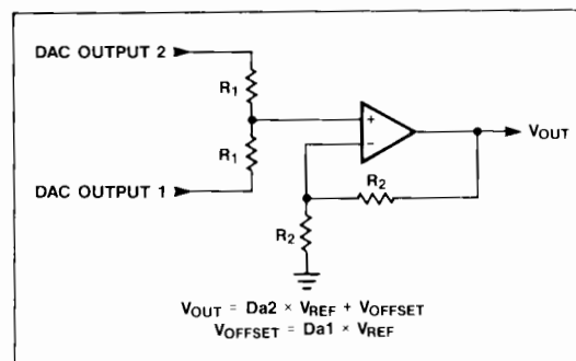
Figure 10. Offset Circuit
