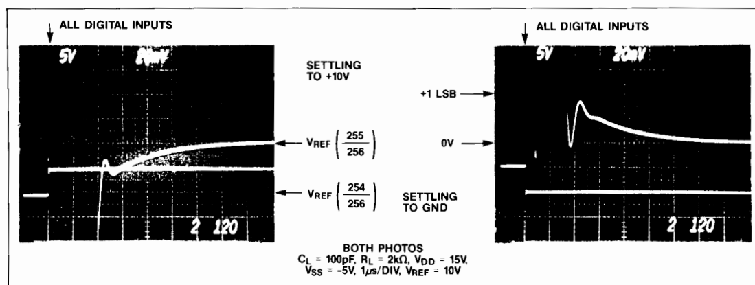
Figure 4. Dynamic Response
