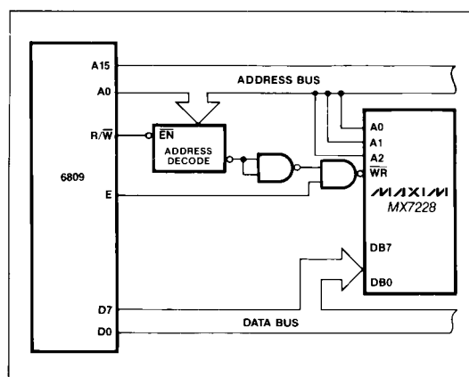
Figure 14. MX7228 to 6809 Interface
