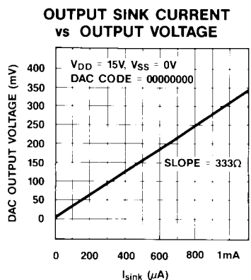
Figure 6. Output Sink/Source Current vs. Output Voltage
