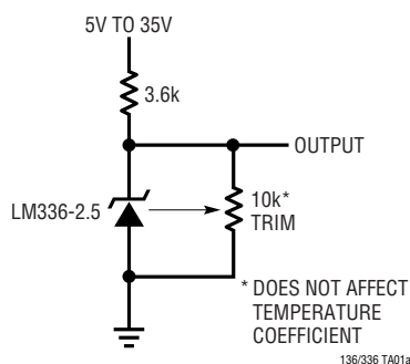
2.5V Reference
