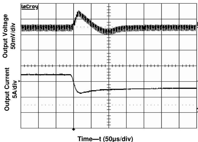
Figure 8. Transient Load Response V_o = 3.3V , V_{in} = 24V , I_o: 3.5A \rightarrow 1.6A , Slew rate 0.1A/\mu s .
