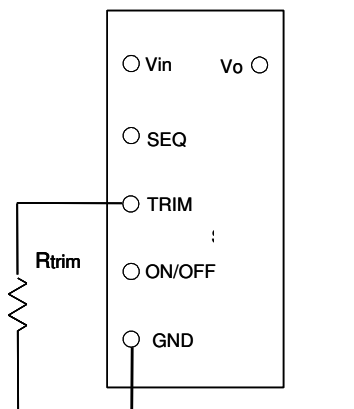
Figure 15. Circuit to Trim Output Voltage
