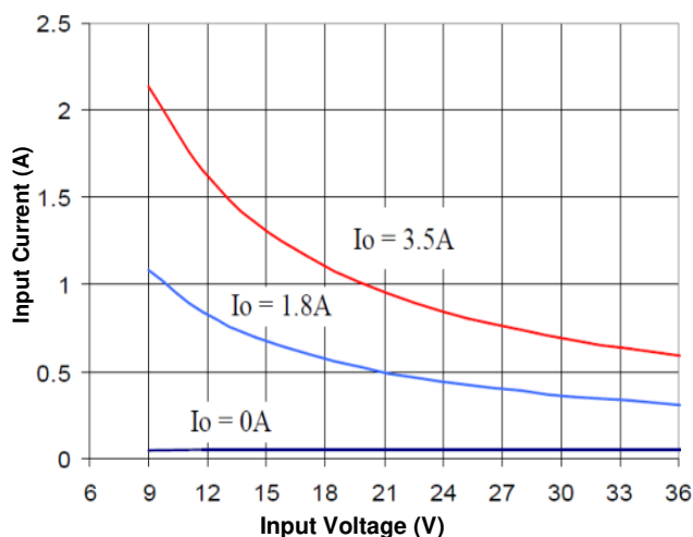
Figure 2. Input Characteristic (5V output)
