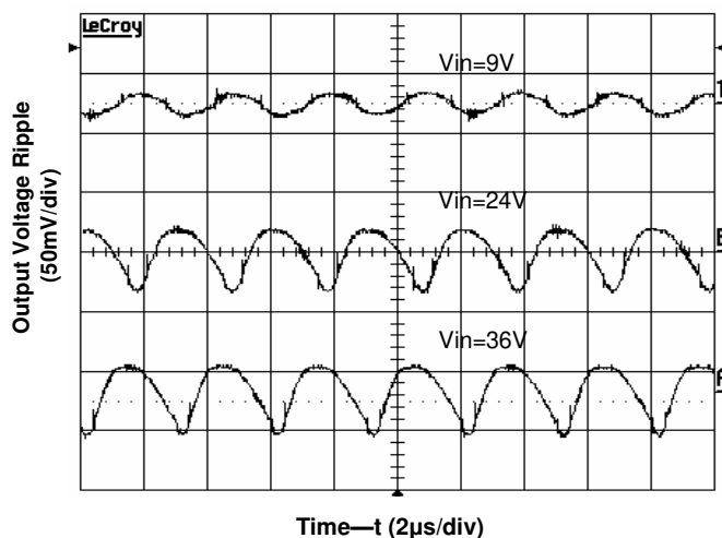
Figure 5. Output Ripple Voltage at 5V, 3.5A Output
