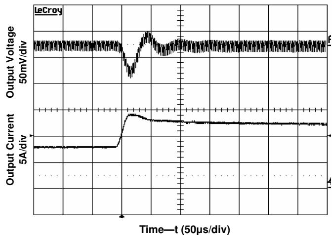
Figure 9. Transient Load Response V_o = 3.3V , V_{in} = 24V , I_o: 1.6A \rightarrow 3.5A , Slew rate 0.1A/\mu s .
