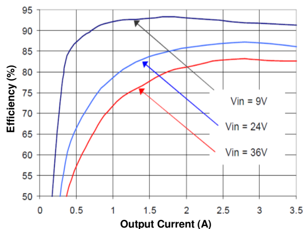
Figure 1(b). Efficiency vs. Load Current (25°C, 5.0V)
