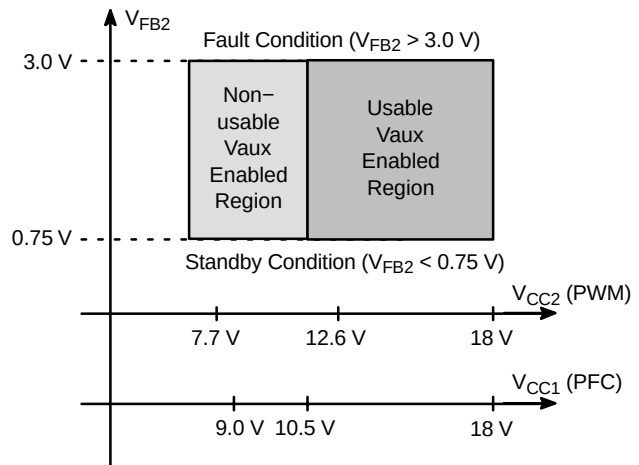
Figure 49. V_{\text{aux}} Enabled Regions
