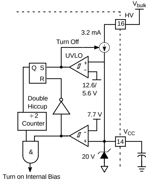
Figure 48. V_{\text{CC2}} Management
