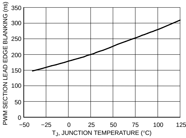
Figure 9. PWM Section Lead Edge Blanking vs. Temperature
