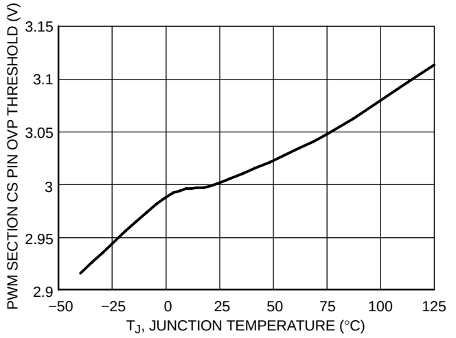
Figure 12. CS2 Pin Overvoltage Protection Threshold vs. Temperature
