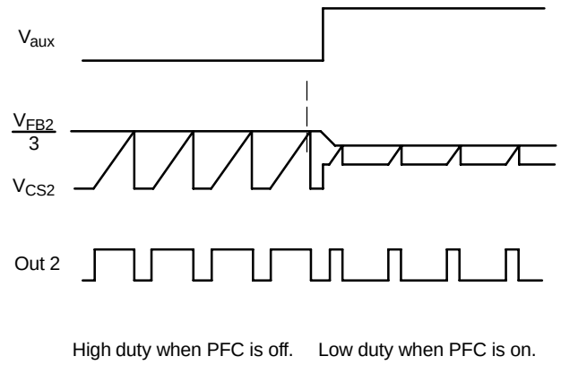
Figure 77. Timing Diagram of PWM Stage When R_{FF} is Added
