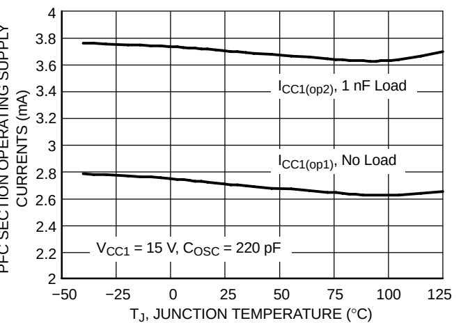
Figure 44. PFC Section Operating Supply Currents vs. Temperature
