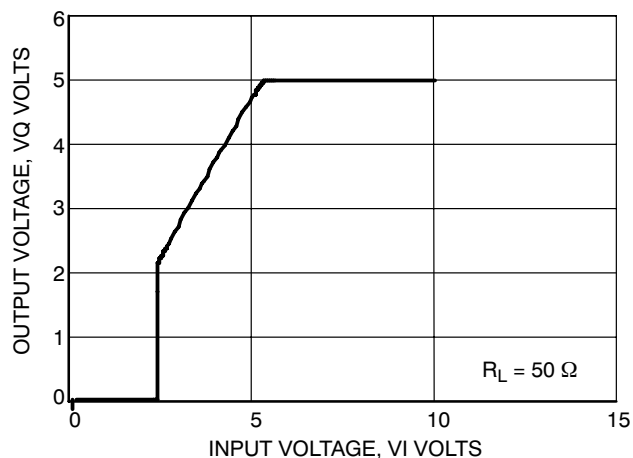
Figure 5. Output Voltage VQ vs. Input Voltage
