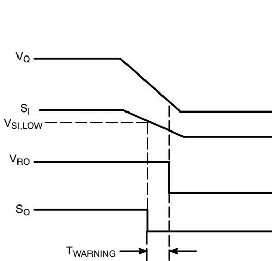
Figure 42. SO Warning Timing Waveform
