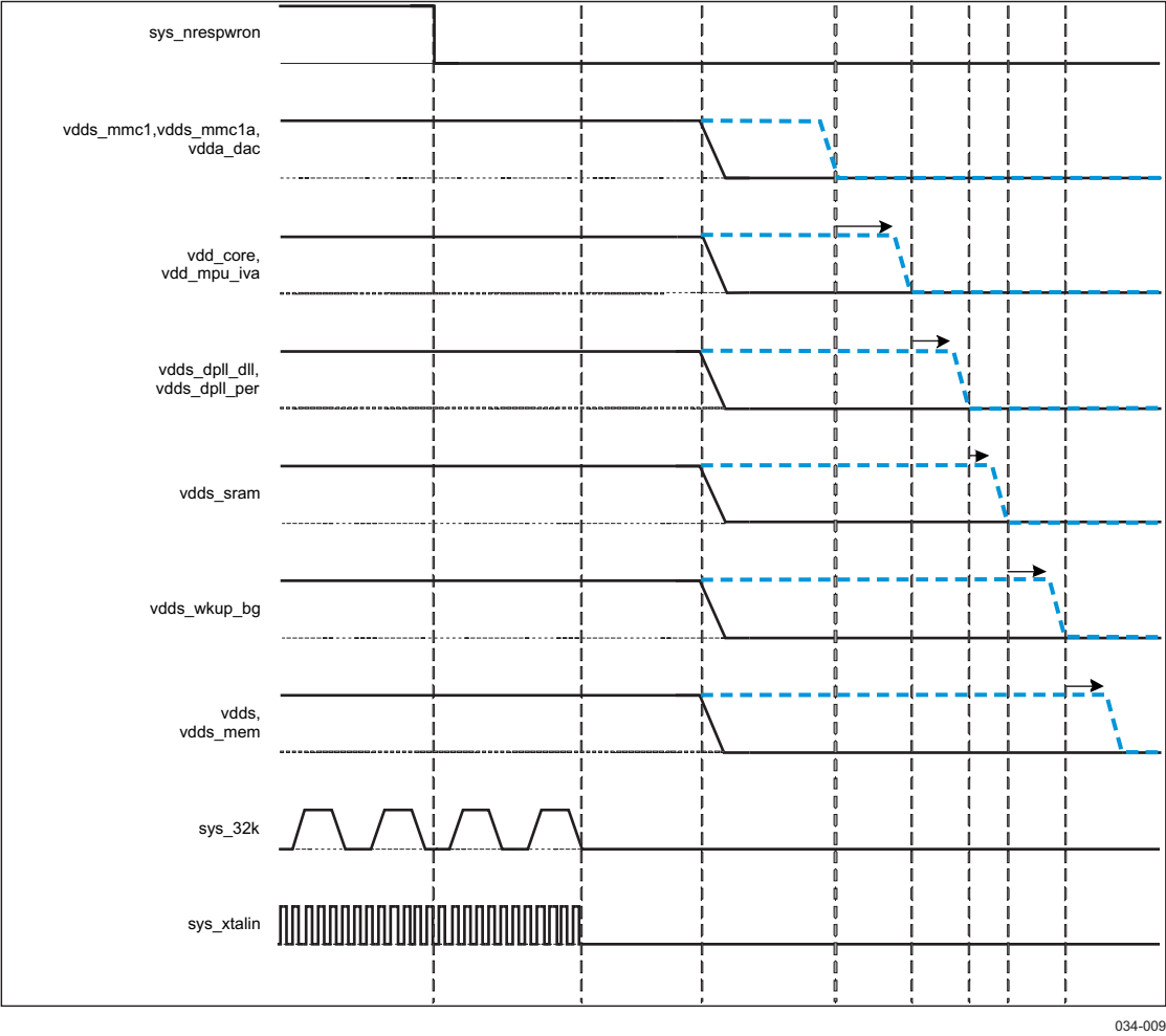
Figure 3-4. Power-down Sequence
