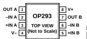
Figure 2. 8-Lead SOIC_N (S Suffix)
