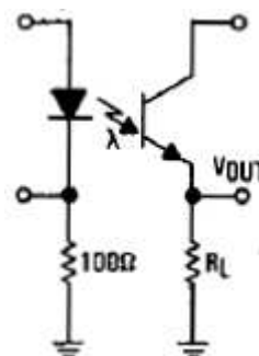
Test Circuit
