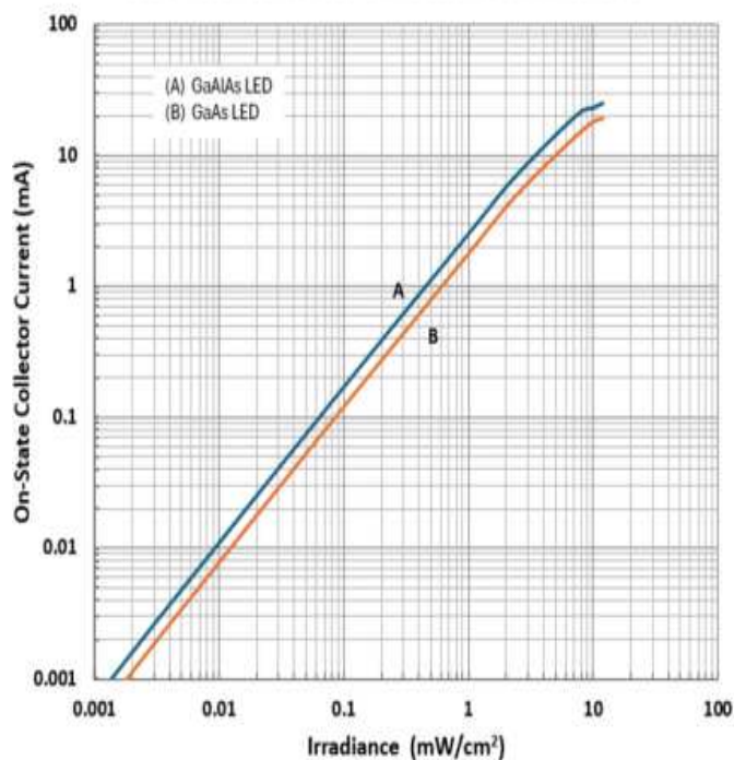
On-State Collector Current vs Irradiance
