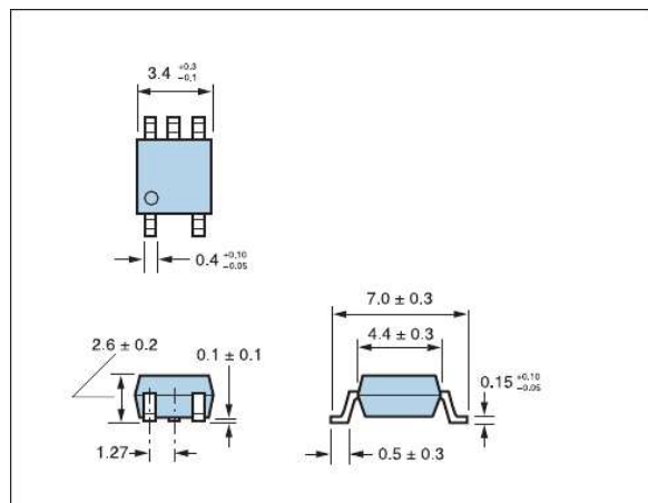
SOP5 1.27mm pin pitch
