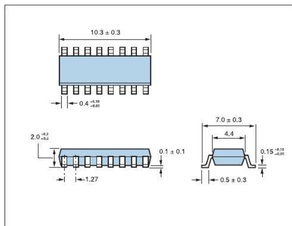
SSOP16 1.27mm pin pitch
