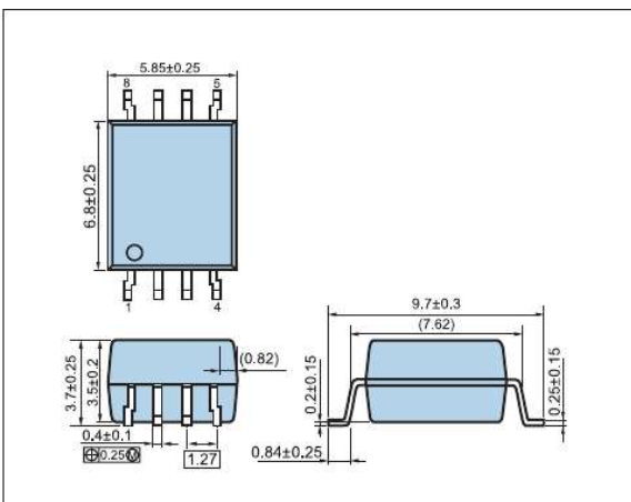
8-Pin SDIP
