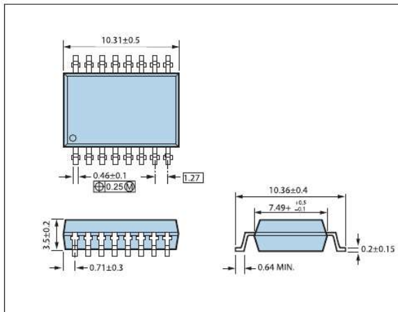
16-Pin SSOP
