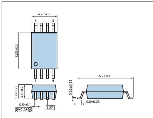
8-Pin LSDIP
