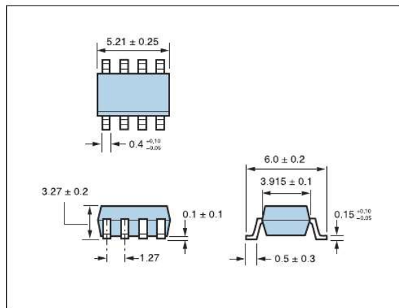
S08 1.27mm pin pitch
