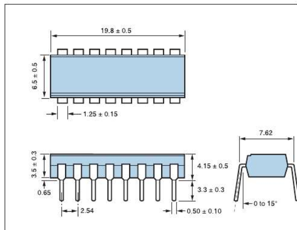
DIP16 Thru-Hole
