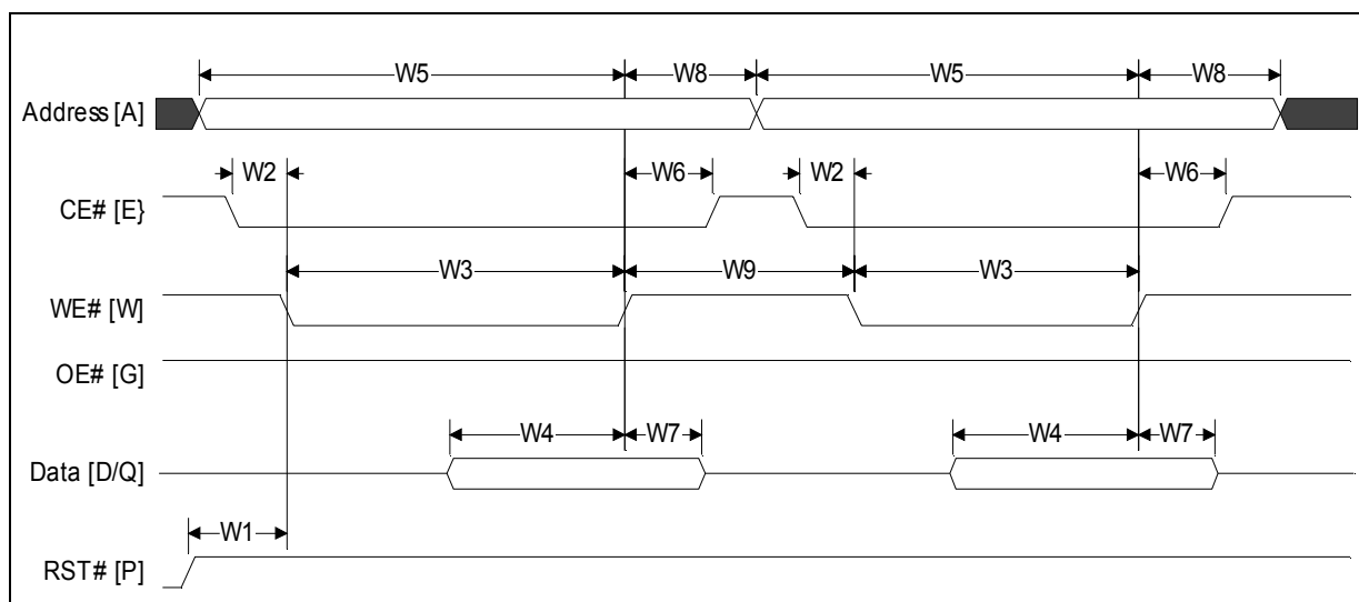
Figure 27: Write-to-Write Timing
