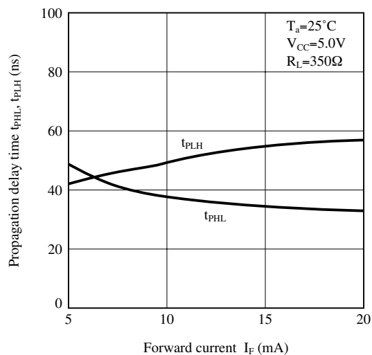
Fig.11 Propagation Delay Time vs. Forward Current
