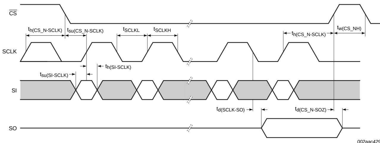
Fig 16. Detailed SPI-bus timing
