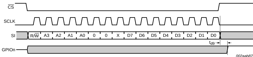
Fig 17. SPI write IOState to GPIO switch
