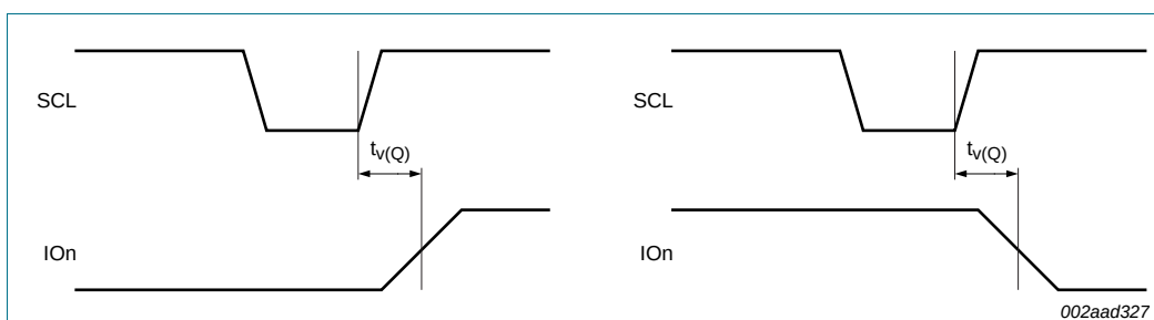
Fig 22. t_{V(Q)} timing
