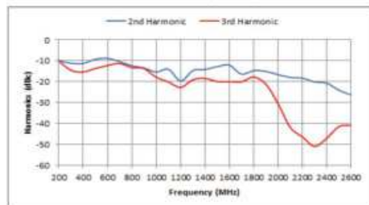
Harmonics (@ Psat)
