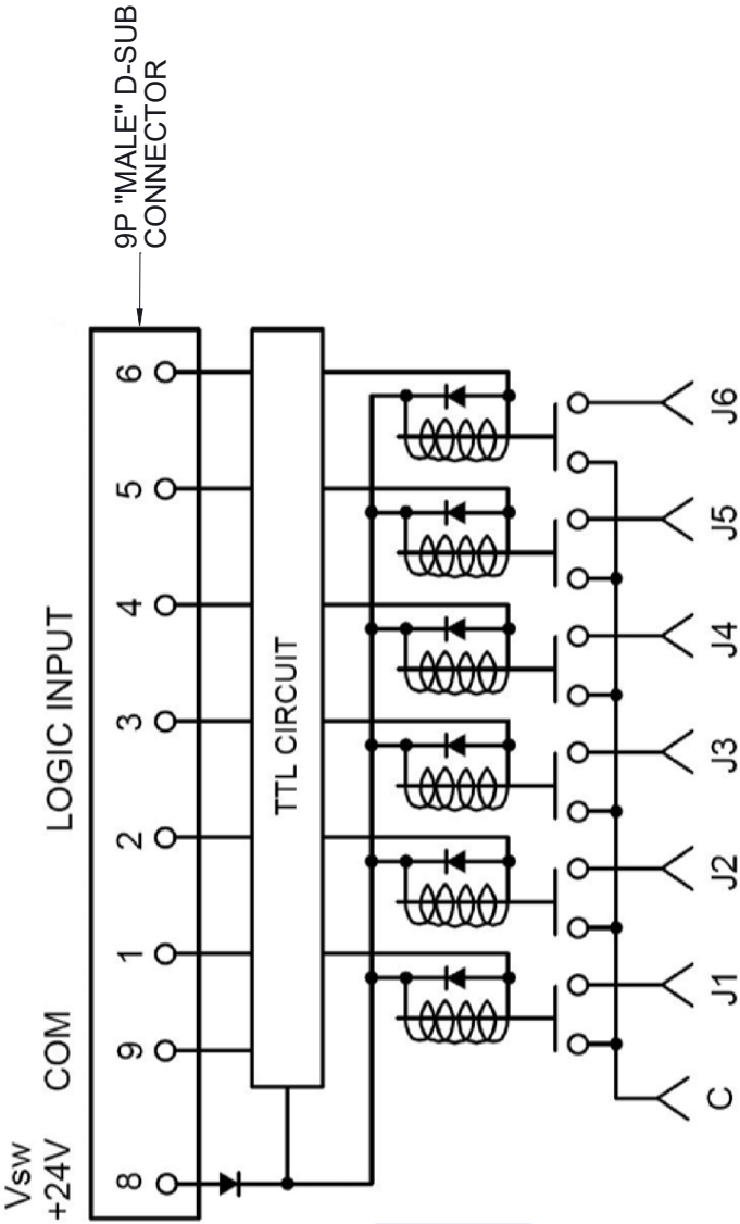
SCHEMATIC SHOWN IN NORMALLY OPEN POSITION
