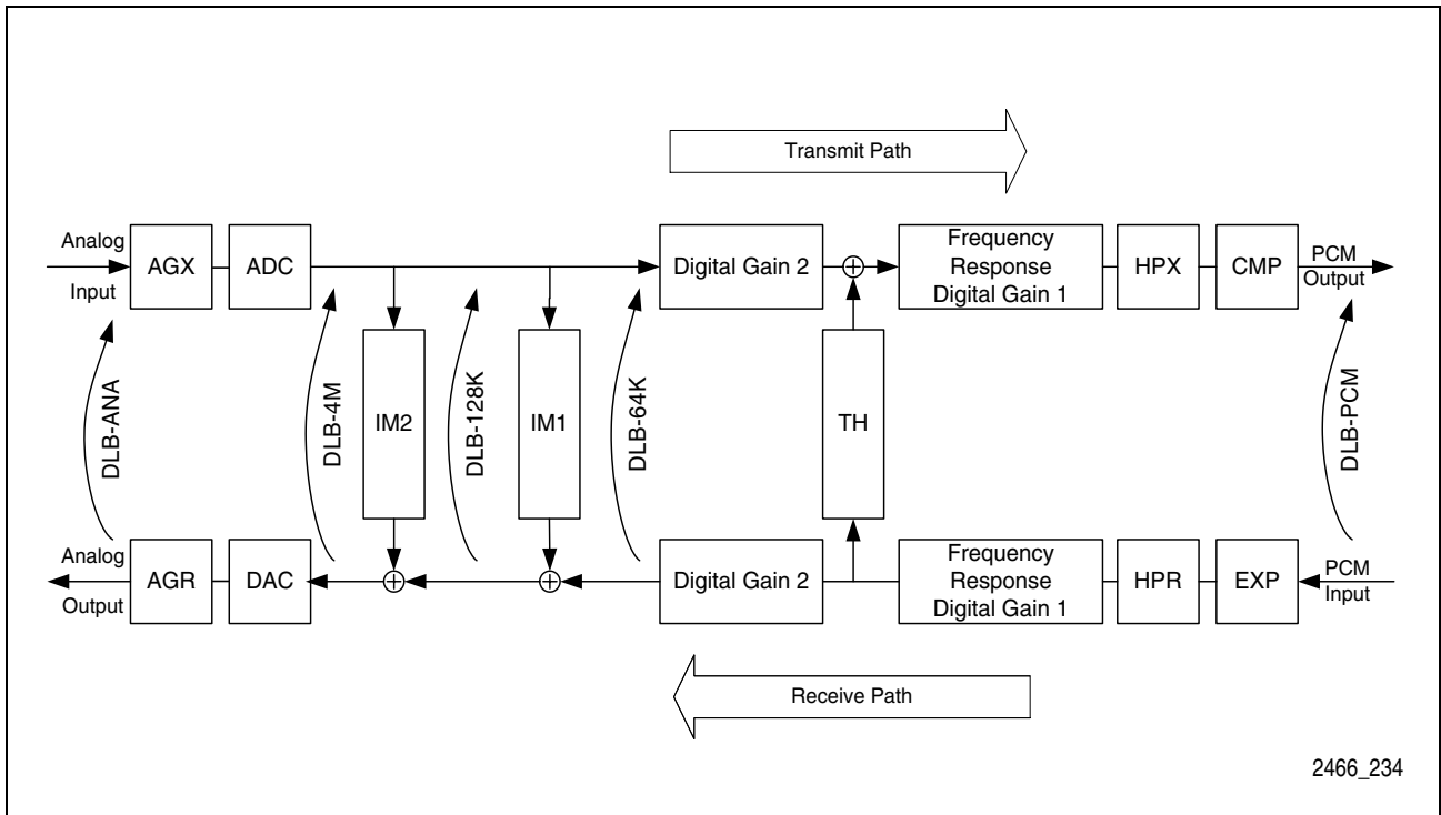
Figure 34 Digital Loops
