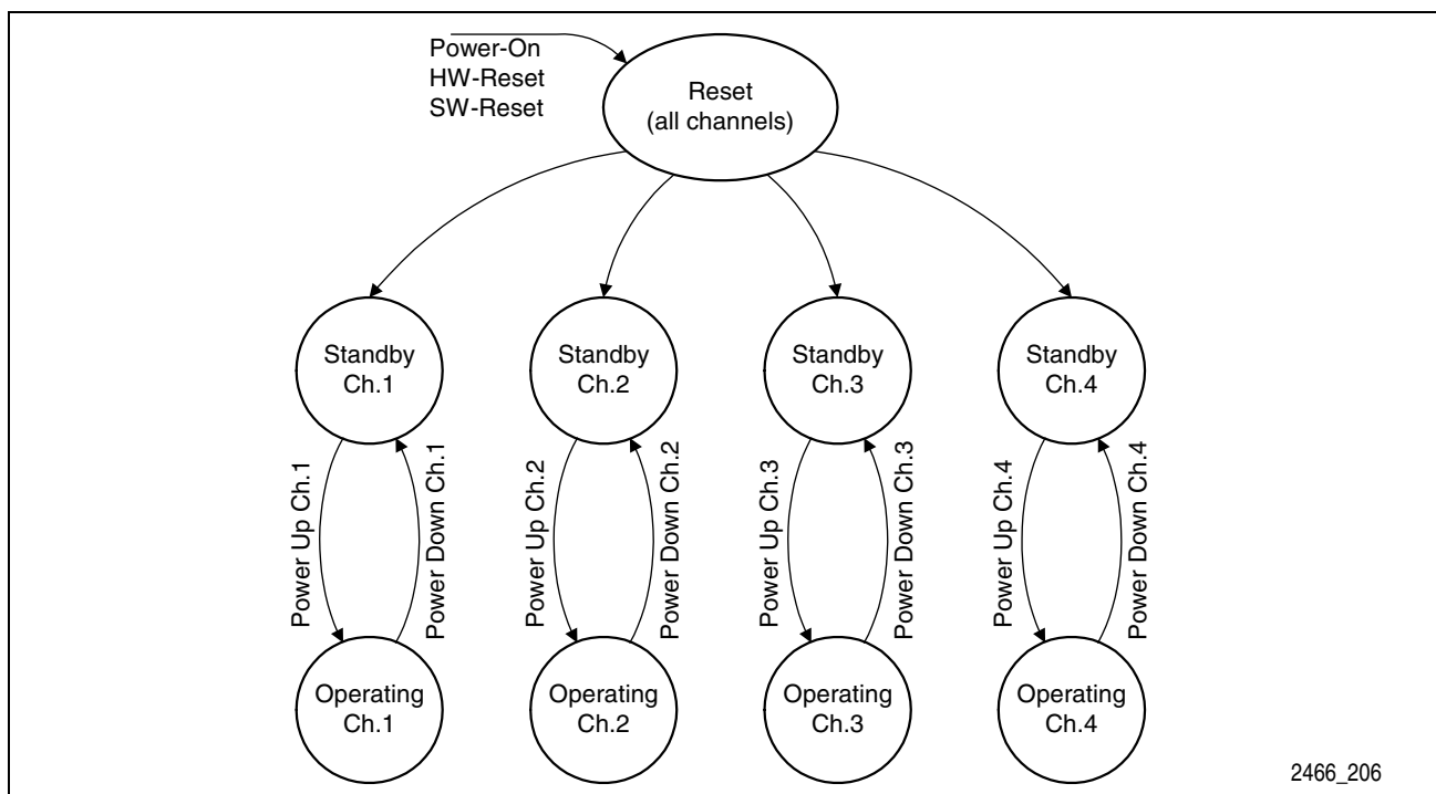
Figure 5 SICOFI®4-μC State Diagram
