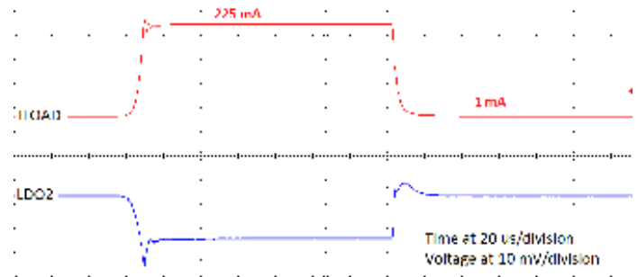
Figure 14. Load transient response - LDO2
