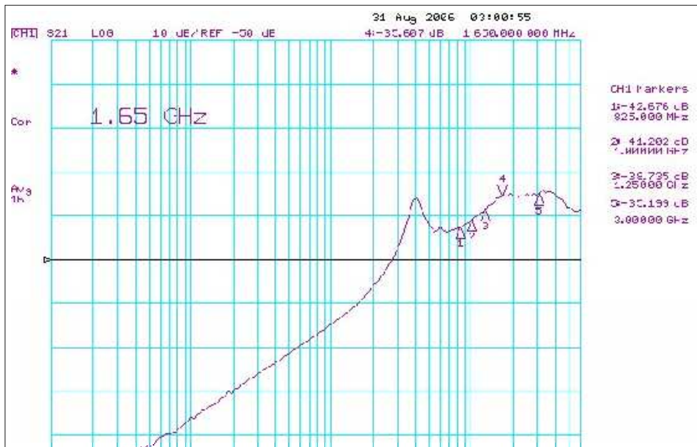
Fig 4. Off Isolation
