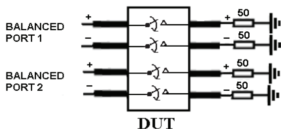
Differential Near End Crosstalk Test Circuit
