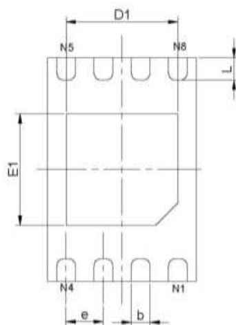
BOTTOM VIEW
