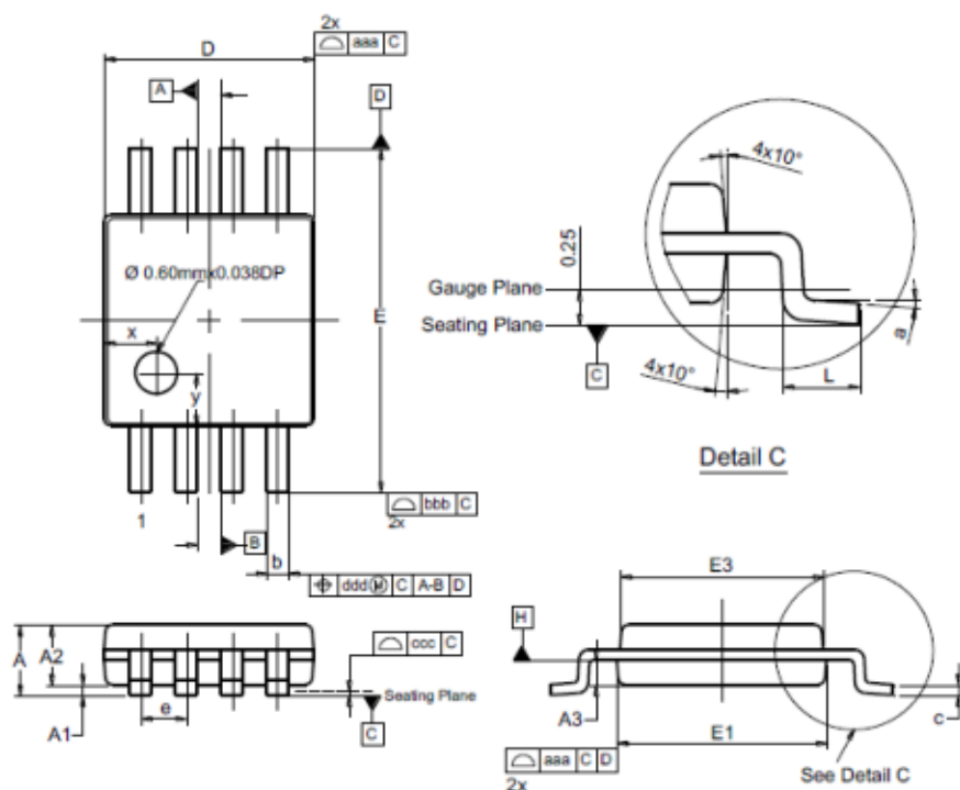
MSOP-8
