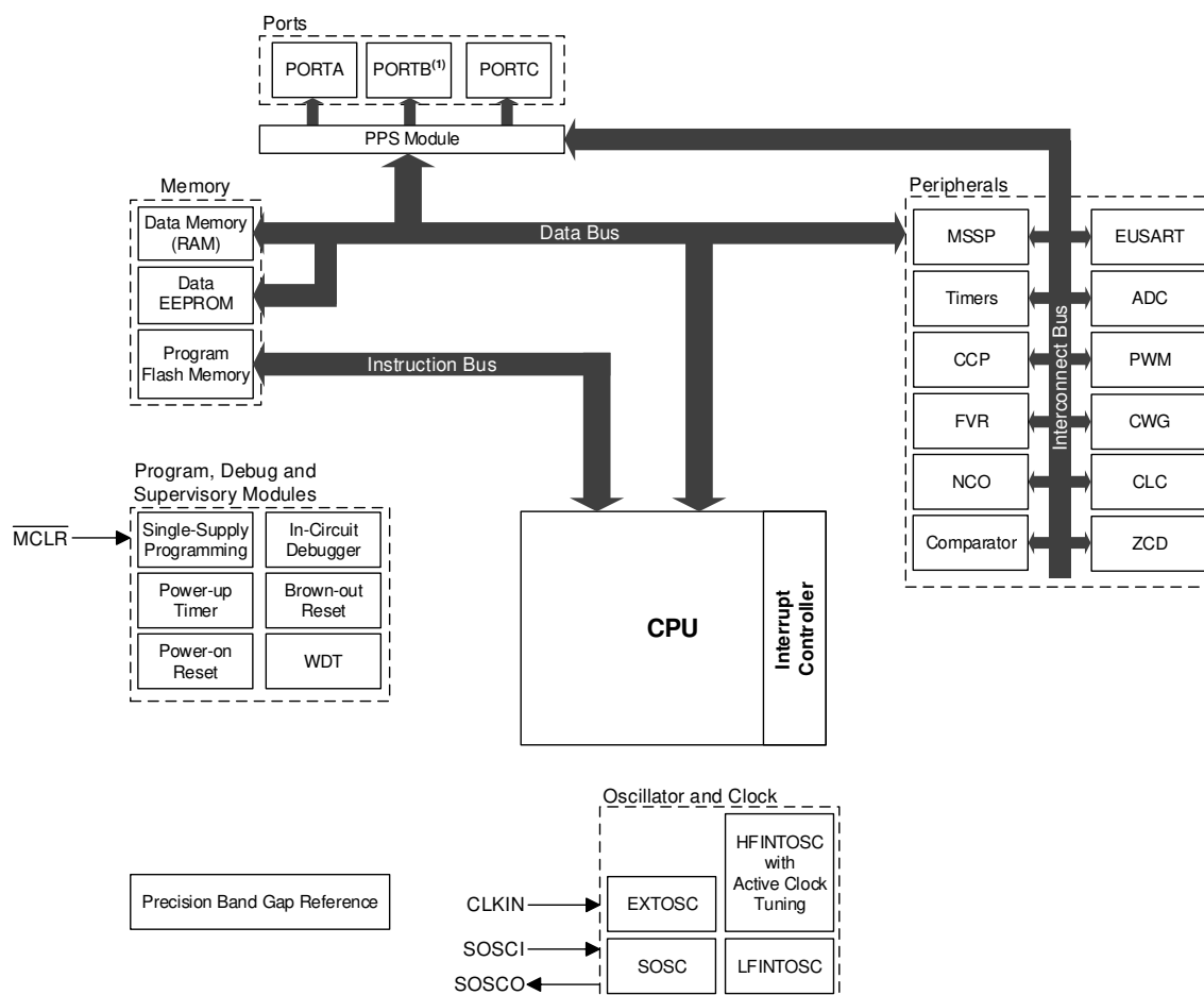
Figure 1. PIC16F18026/46 Block Diagram
