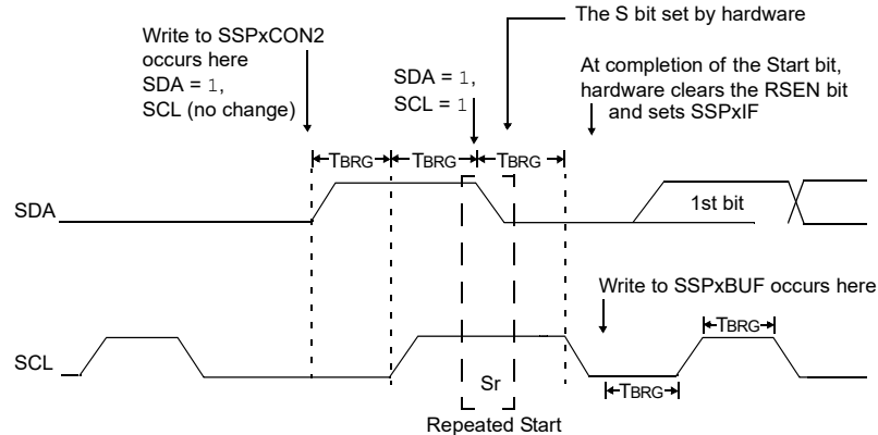
Figure 29-26. Repeated Start Condition Waveform
