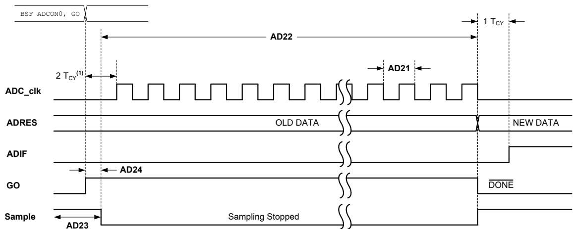
Figure 41-11. ADC Conversion Timing (ADC Clock from ADCRC)
