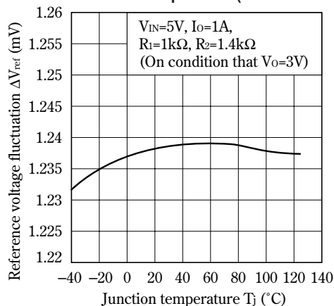
Fig.7 Reference Voltage Fluctuation vs. Junction Temperature (PQ150VB02FZ)
