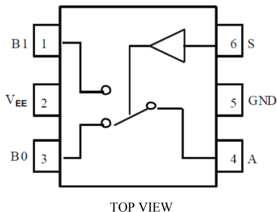
Figure 1. 6-lead SC70
