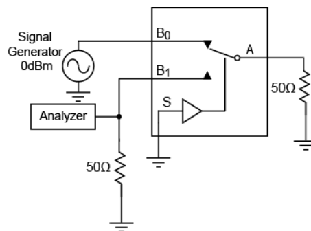
Figure 7. Crosstalk
