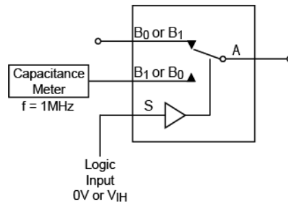
Figure 8. Channel Off Capacitance
