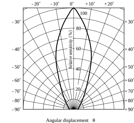
Fig. 9 Sensitivity Diagram ( T_a = 25^{\circ}C )
