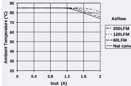
Safe Operating Area @ V_{in} = 48\text{V} (Note B)
