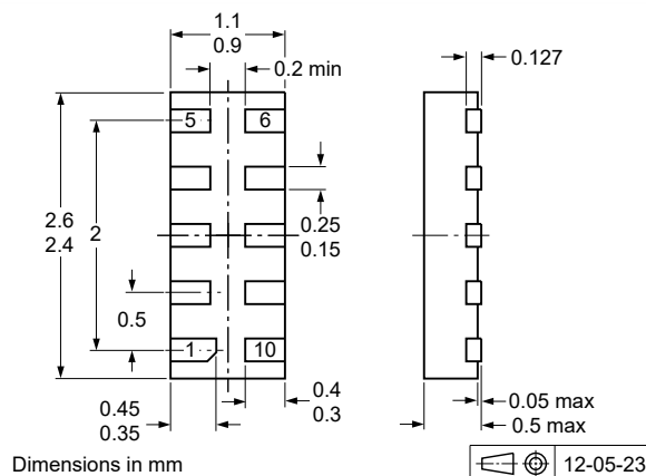
Fig. 15. Package outline DFN2510A-10 (SOT1176-1)
